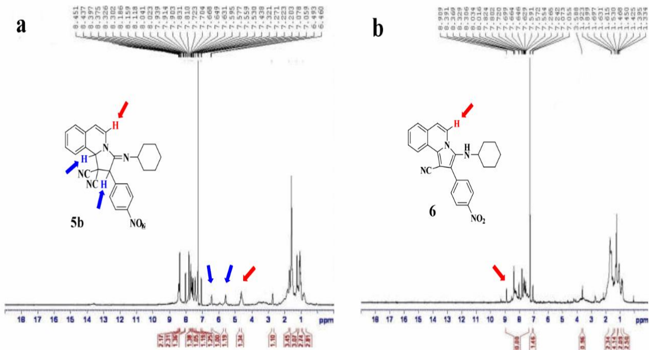
Fig. 1. ^1\text{H} NMR spectra of products (5b) (a) and (6a) (b).
